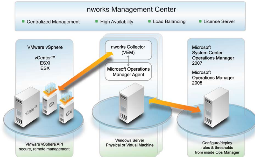
Management integration with nworks Management Pack and VMware vCenter™
